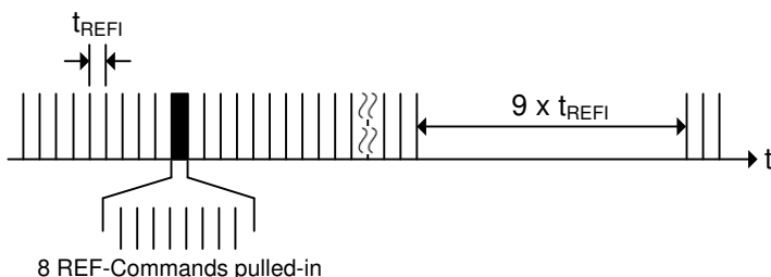
Figure 30. Pulling-in Refresh Commands (Example)
