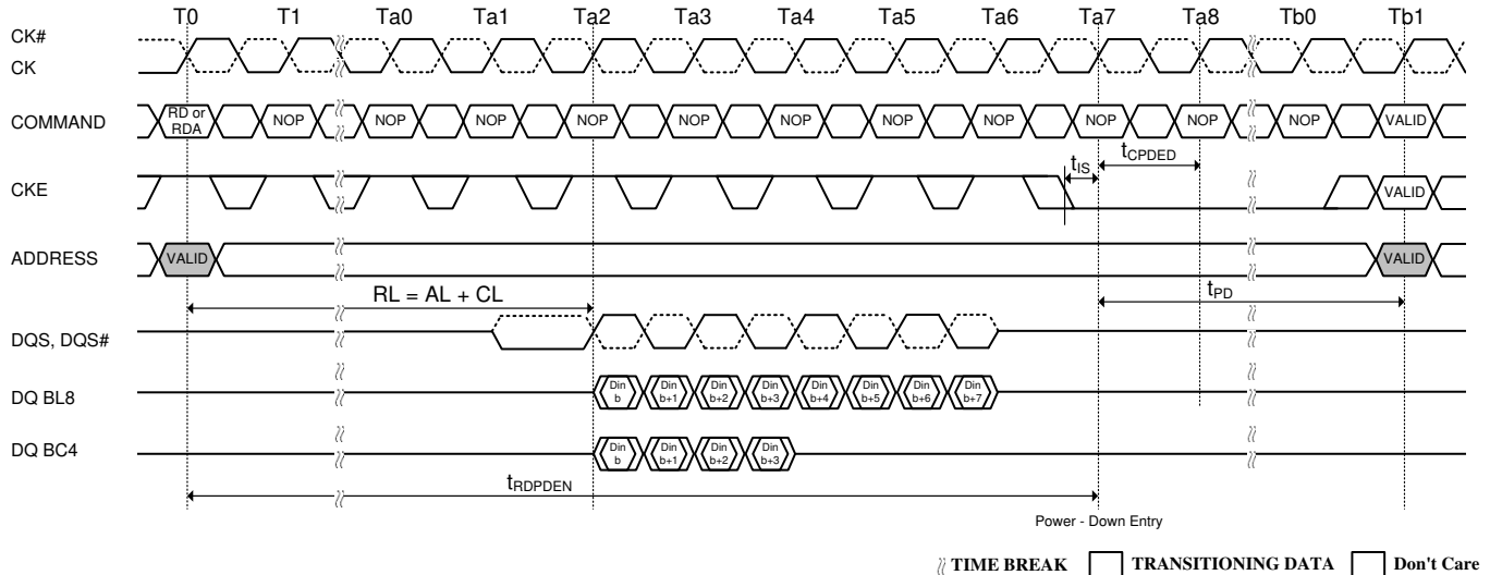
Figure 80. Power-Down Entry after Read and Read with Auto Precharge
