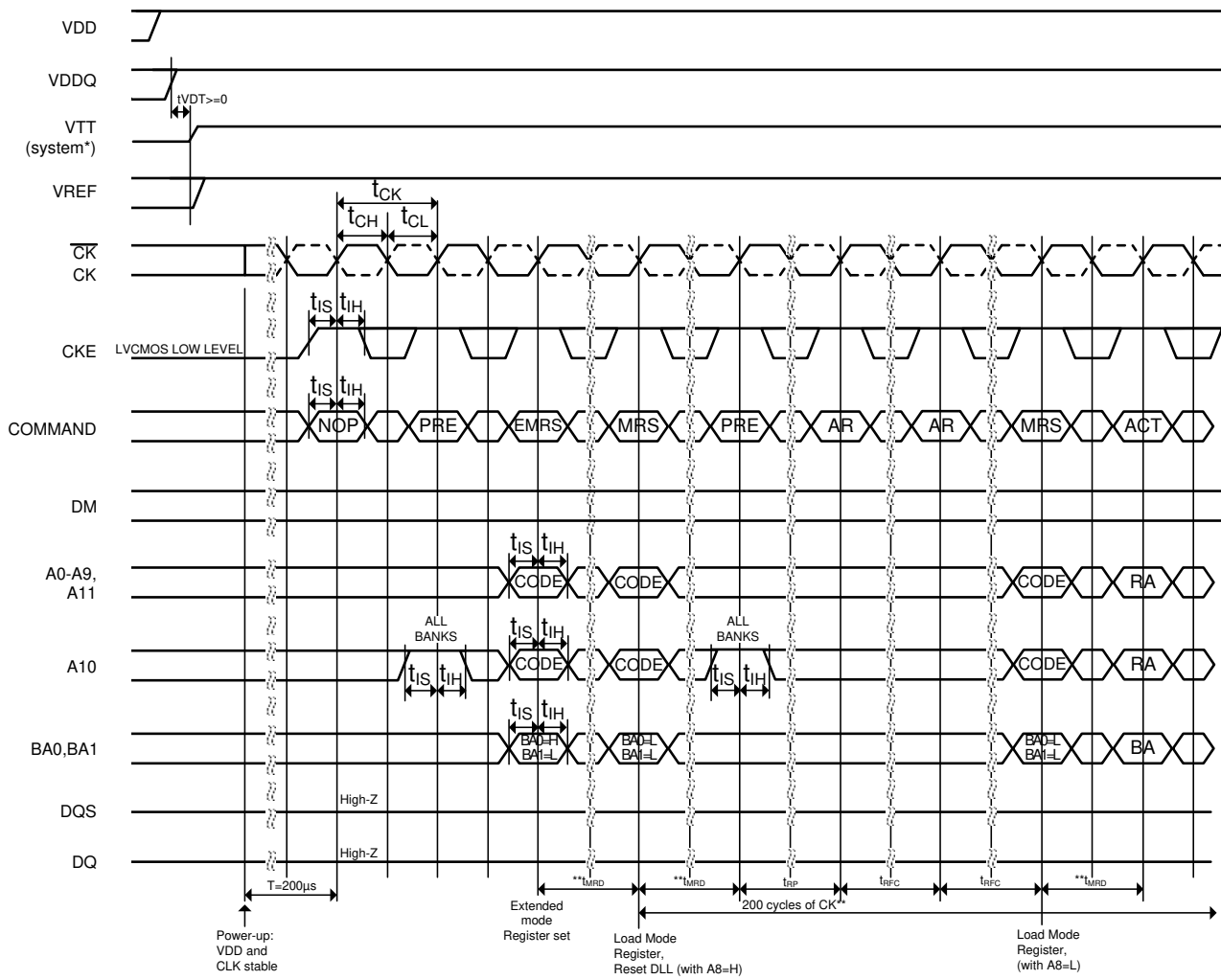
Figure 48. Initialize and Mode Register Sets
