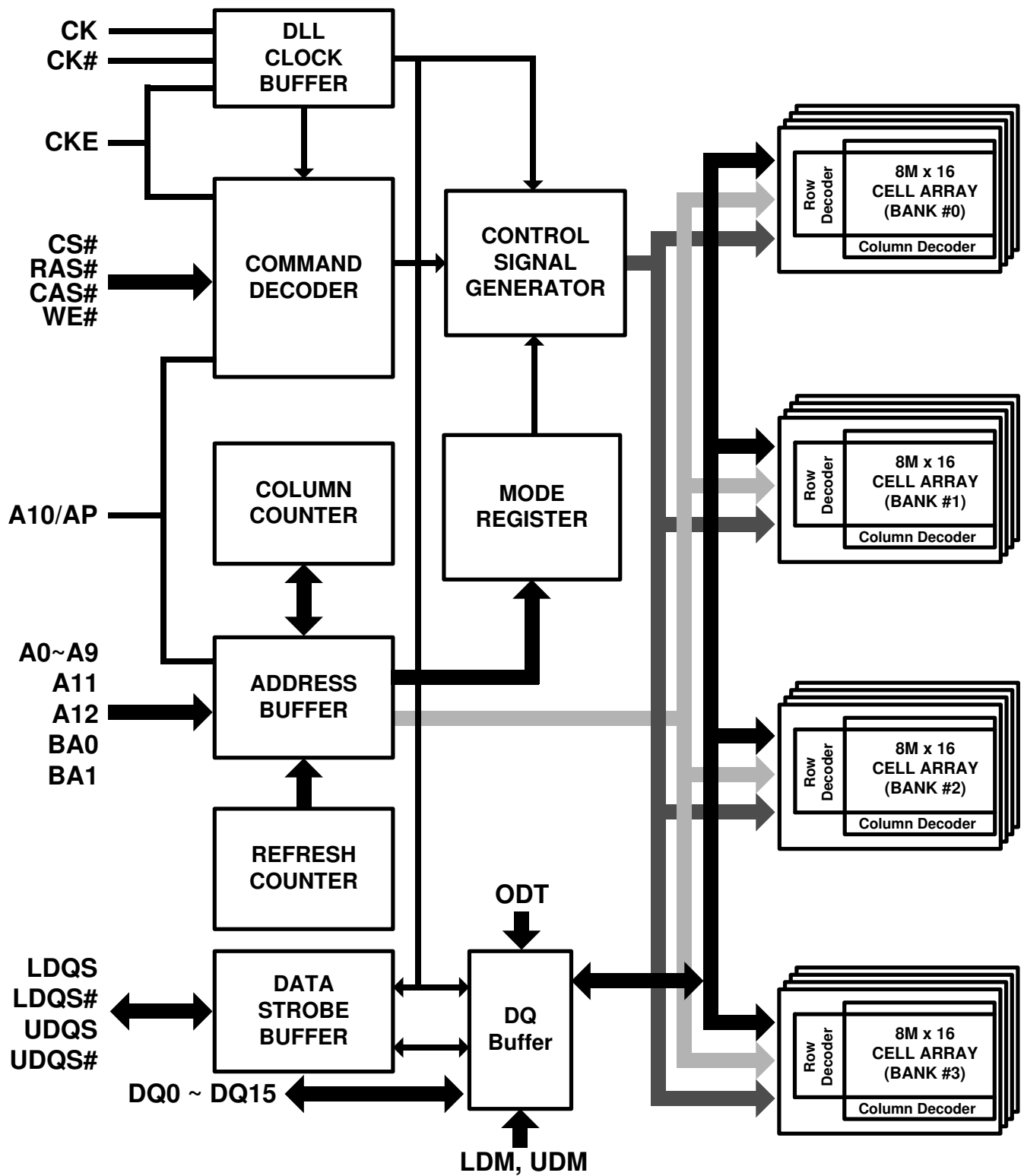
Figure 2. Block Diagram
