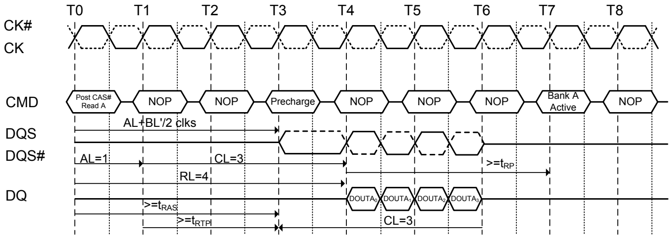
Figure 30.1. Burst read operation followed by precharge: (RL=4, AL=1, CL=3, BL=4, t_{RTP} \square 2 clocks)
