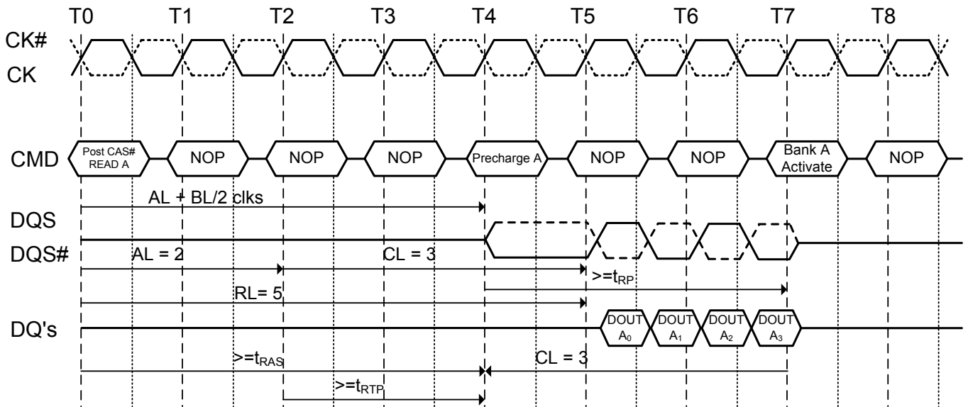
Figure 30.3. Burst read operation followed by precharge: (RL=5, AL=2, CL=3, BL=4, t_{RTP} \square 2 clocks)
