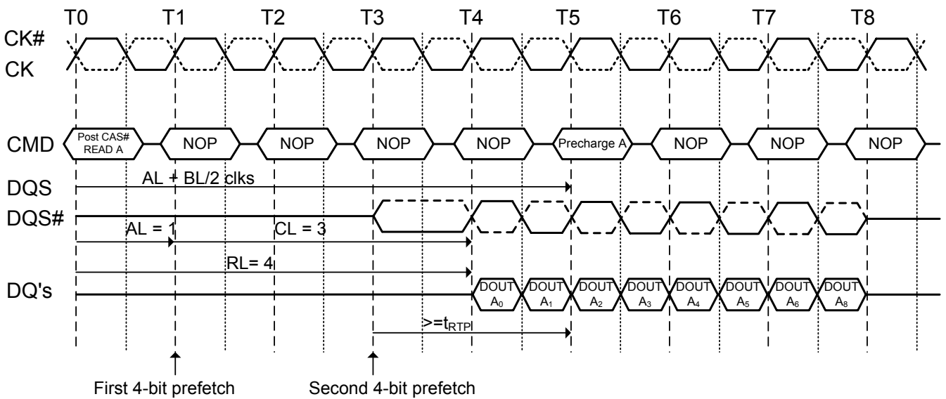
Figure 30.2. Burst read operation followed by precharge: (RL=4, AL=1, CL=3, BL=8, t_{RTP} \square 2 clocks)
