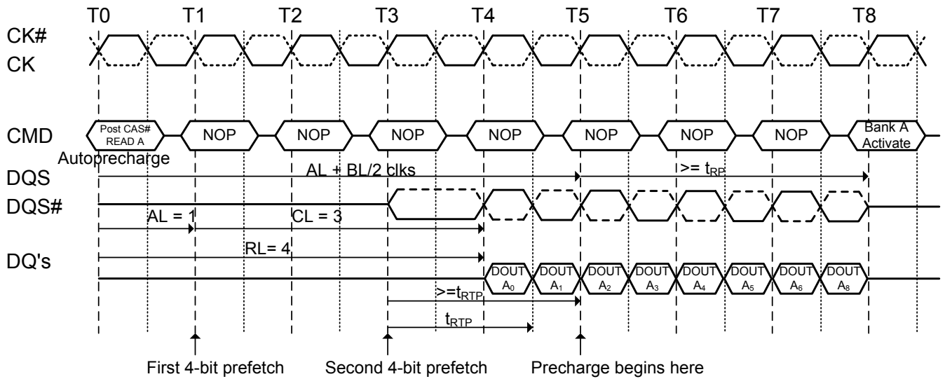
Figure 32.1. Burst read operation with auto precharge: ( RL=4, AL=1, CL=3, BL=8, t_{RTP} \square 2 clocks)
