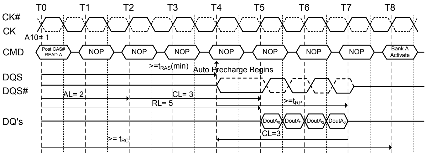
Figure 32.3. Burst read operation with auto precharge followed by activation to the same bank ( t_{RC} Limit): RL=5(AL=2, CL=3, internal t_{RCD}=3 , BL=4, t_{RTP} \leq 2 clocks)
