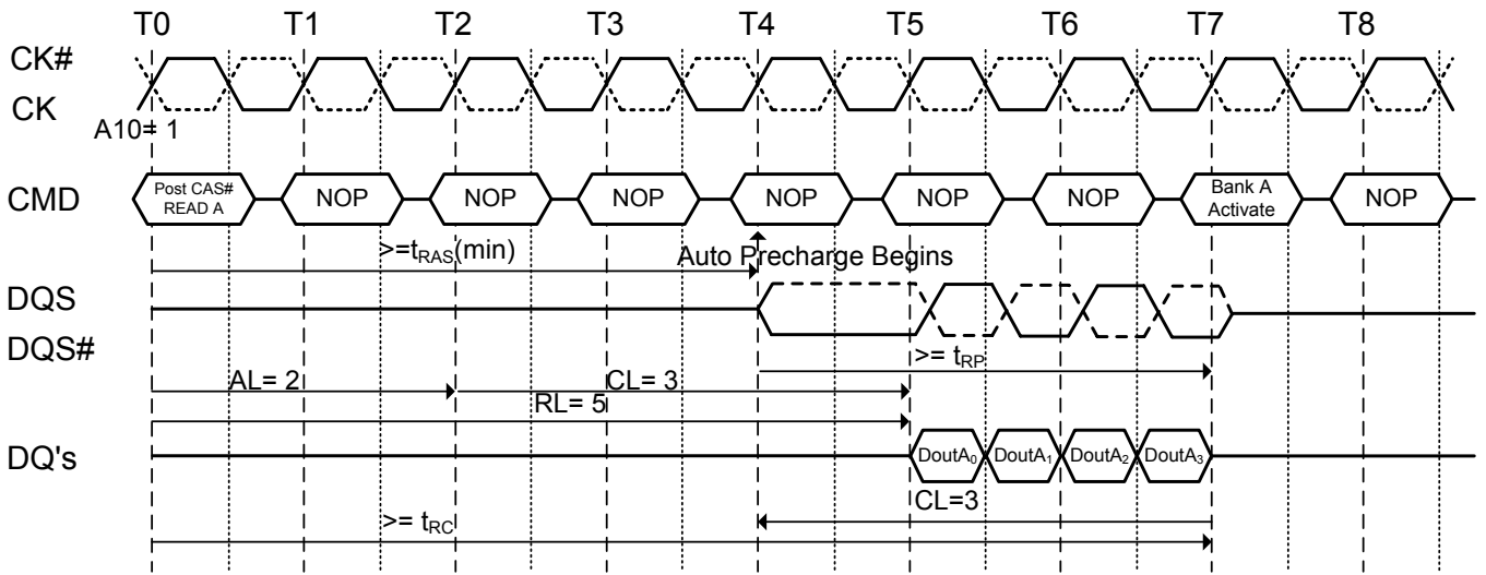
Figure 32.4. Burst read operation with auto precharge followed by an activation to the same bank ( t_{RP} Limit): (RL=5 (AL=2, CL=3, internal t_{RCD} =3, BL=4, t_{RTP} \square 2 clocks)
