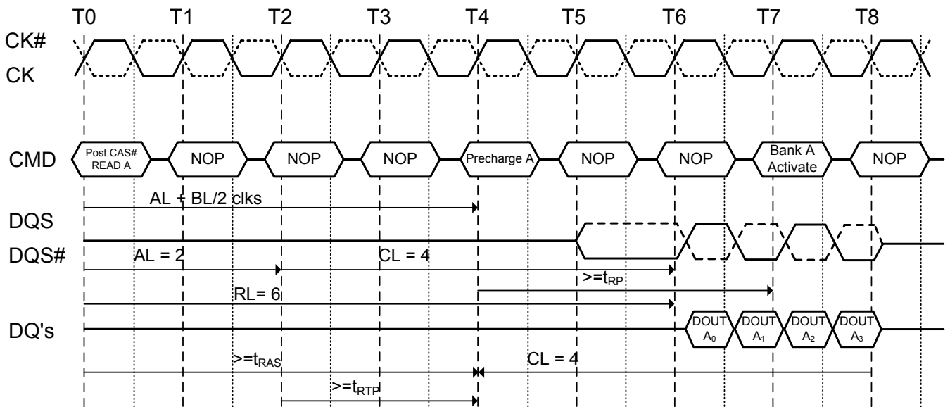
Figure 30.4. Burst read operation followed by precharge: (RL=6, AL=2, CL=4, BL=4, t_{RTP} \square 2 clocks)
